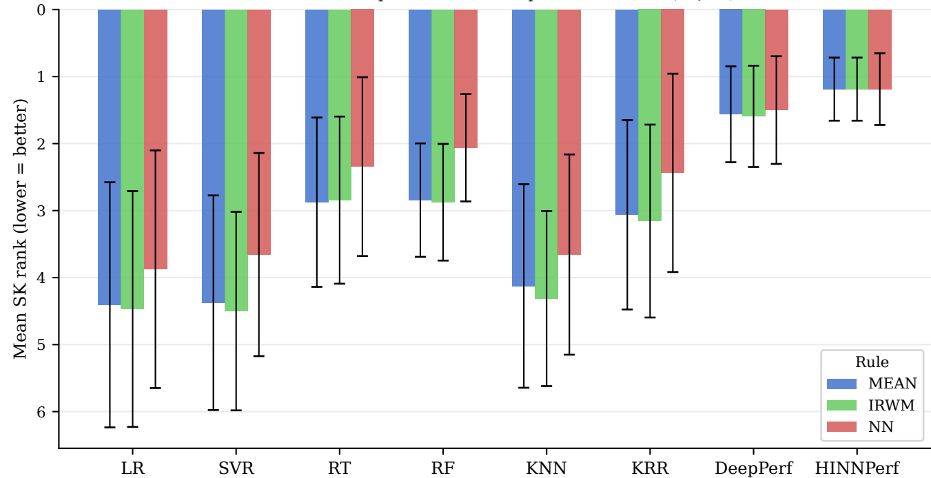
Mean SK rank per rule — best k per scenario, S1 (RQ3.3)
