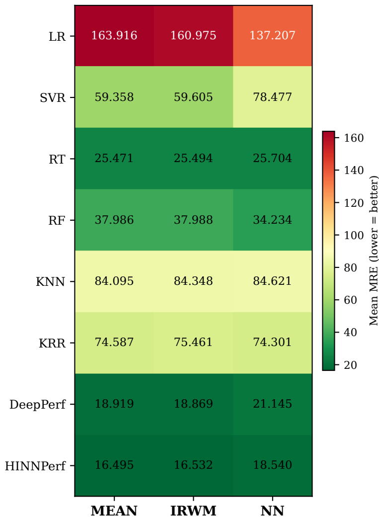
Mean MRE per (base type, rule) — best k per scenario, 40 scenarios (RQ3.3)
