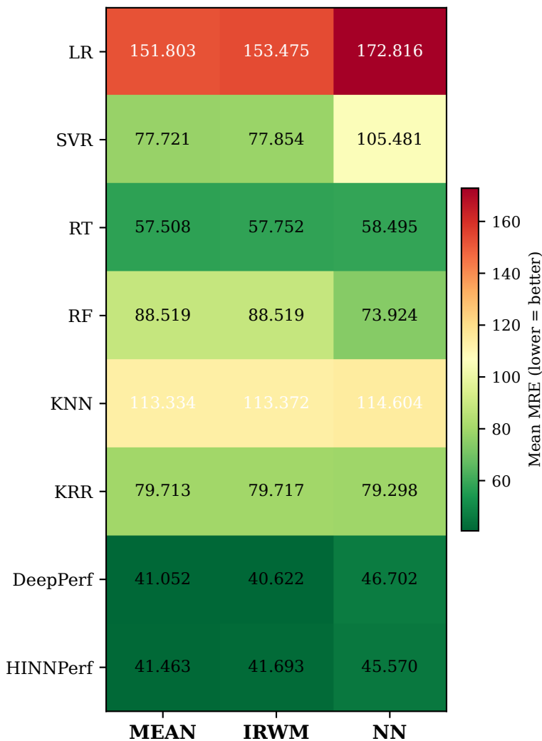
Mean MRE per (base type, rule) — best k per scenario, S1 (RQ3.3)
