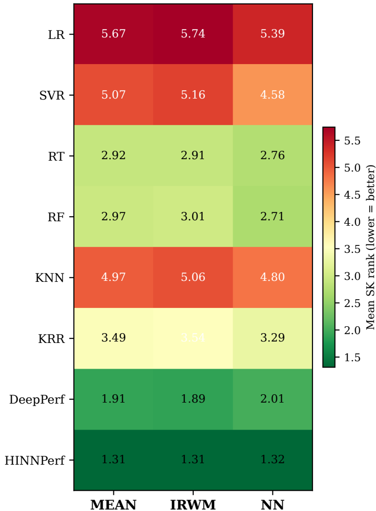
Mean SK rank per (base type, rule) — best k per scenario, 40 scenarios (RQ3.3)
