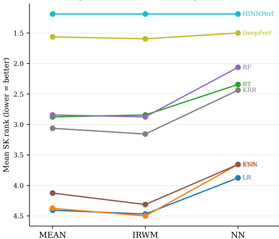
Mean SK rank per combination rule — best k per scenario (RQ3.3, S1)
