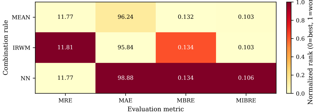
Rule performance by metric — column-normalized (yellow=best, red=worst) Annotated with raw median across all (base type × dataset × sample size) scenarios
