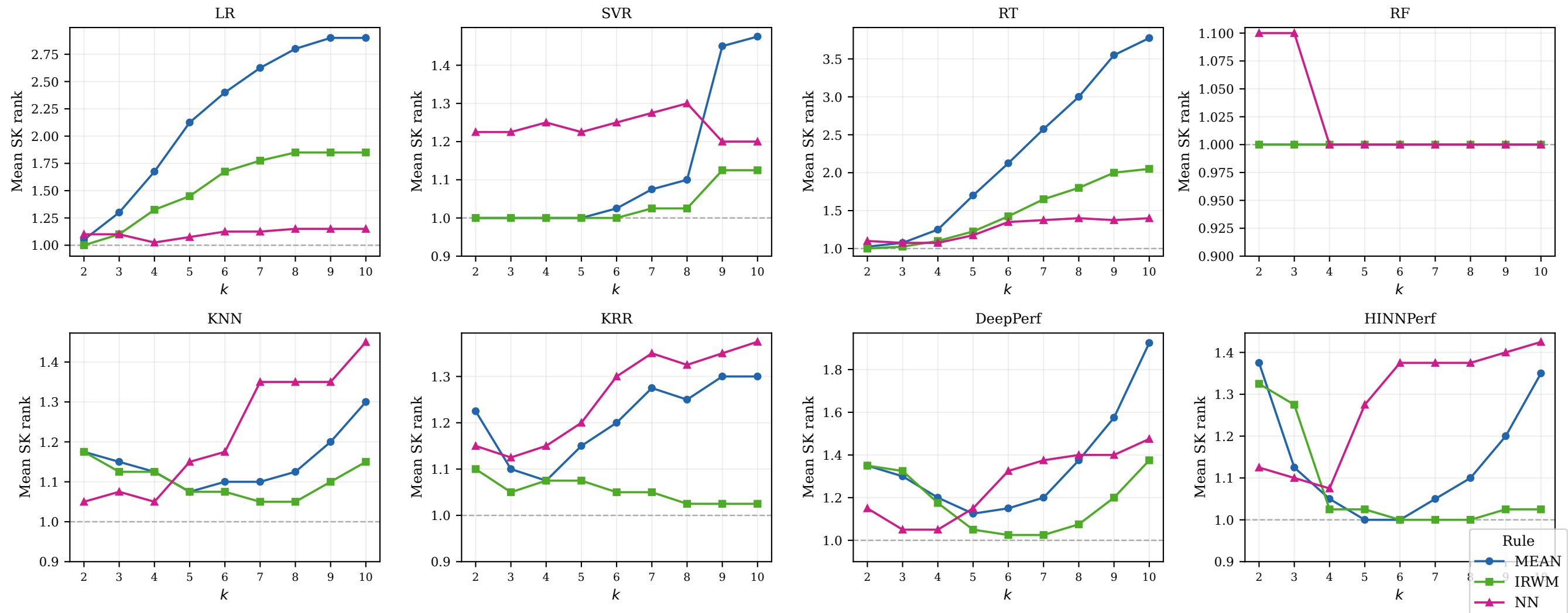
Mean SK rank vs k per base type — all 40 scenarios (RQ3.2) Dashed line at 1 = statistically best group threshold
