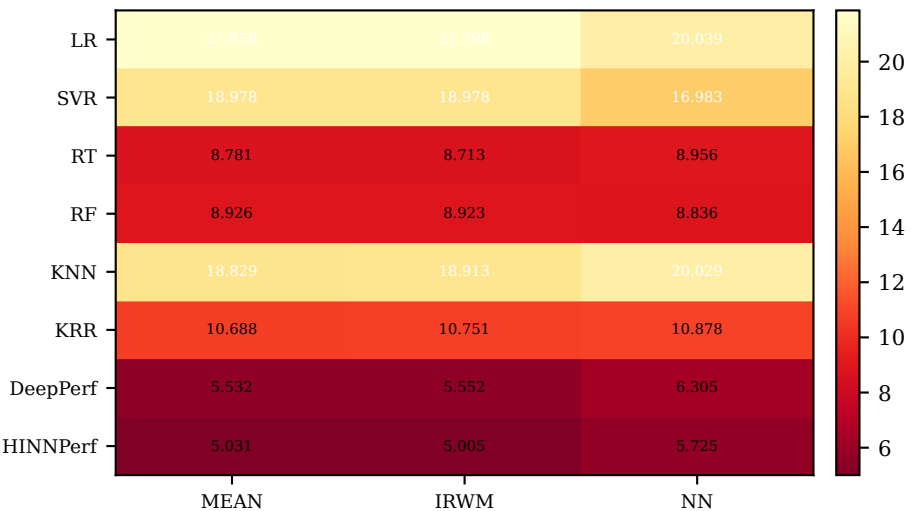
Absolute — MAE
