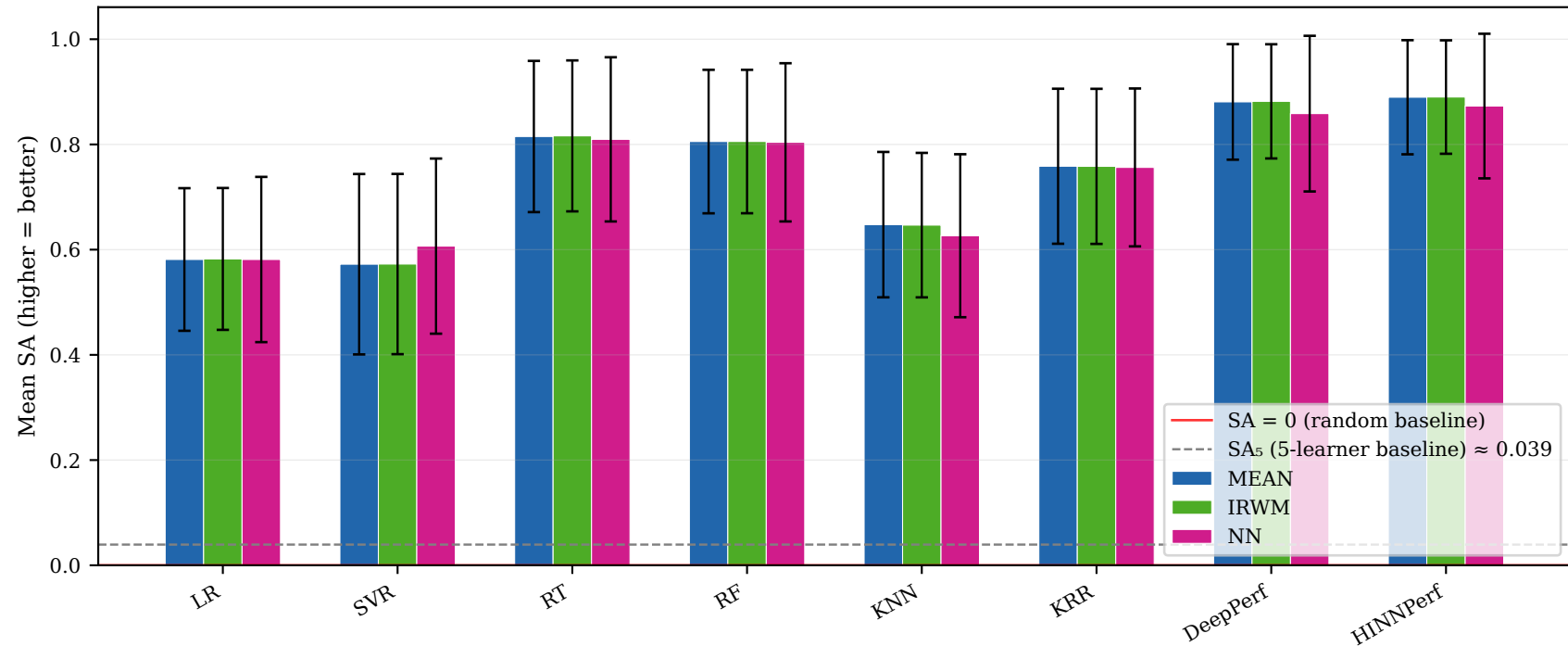
SA by combination rule (RQ3.3) Does MEAN/IRWM beat random more reliably than NN?
