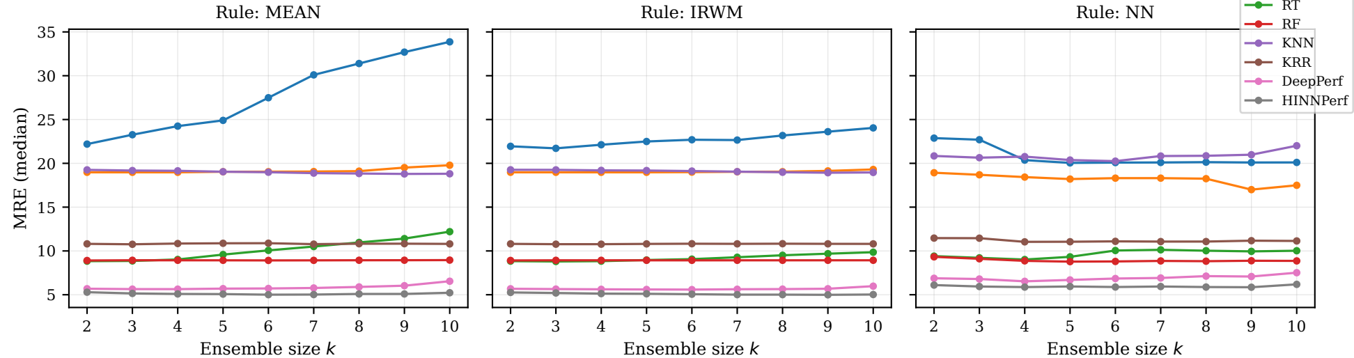
Effect of ensemble size on MRE (median across all datasets)
