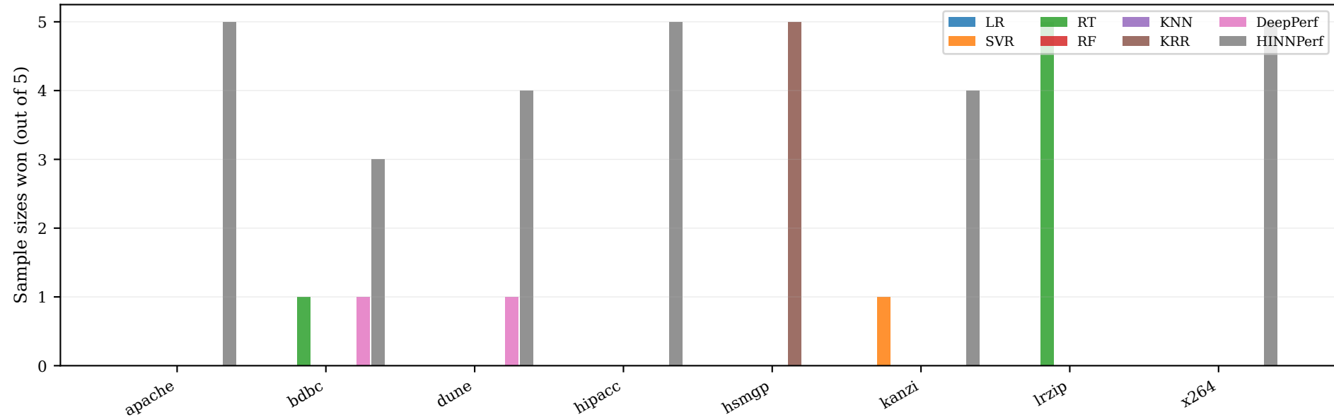
Per-dataset model dominance on MRE — RQ1
