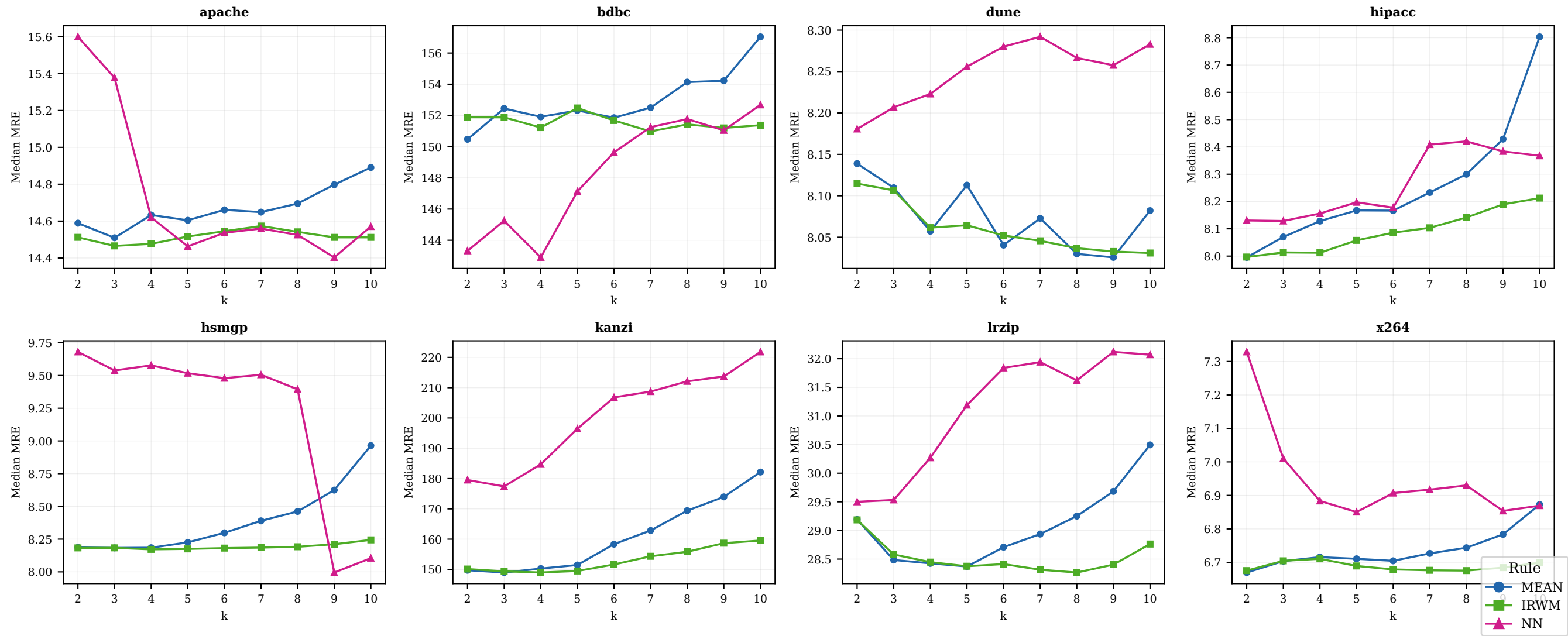
MRE vs k per dataset — aggregated across base types (RQ3.2)
