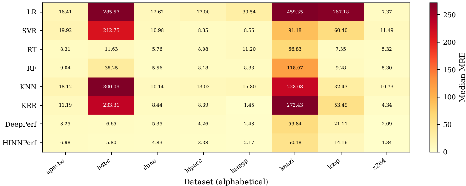
Median MRE per model × dataset (alpha)
