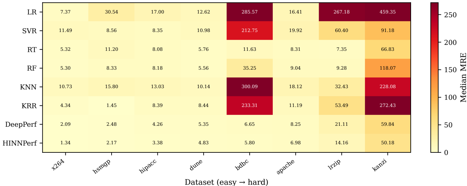
Median MRE per model × dataset (difficulty)
