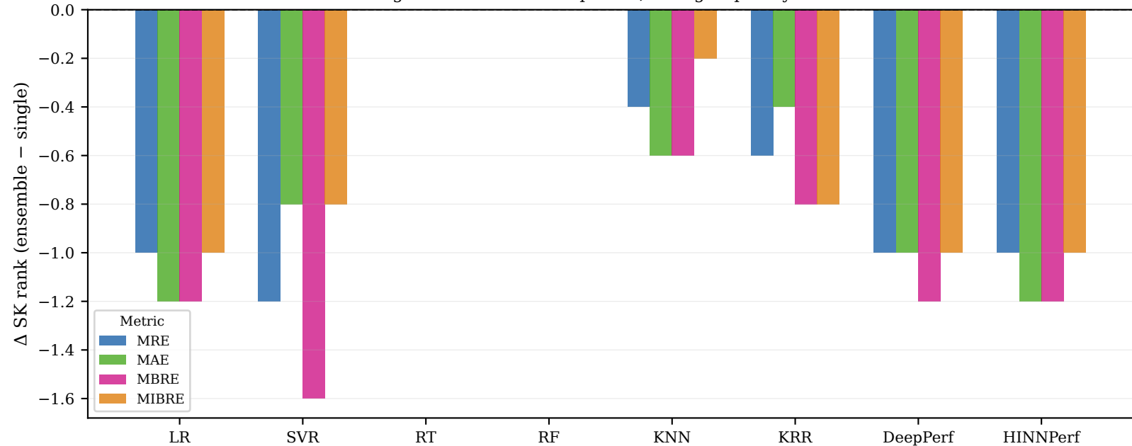
SK rank change: best ensemble vs single — dune (RQ2) Negative = ensemble improved; bars grouped by metric
