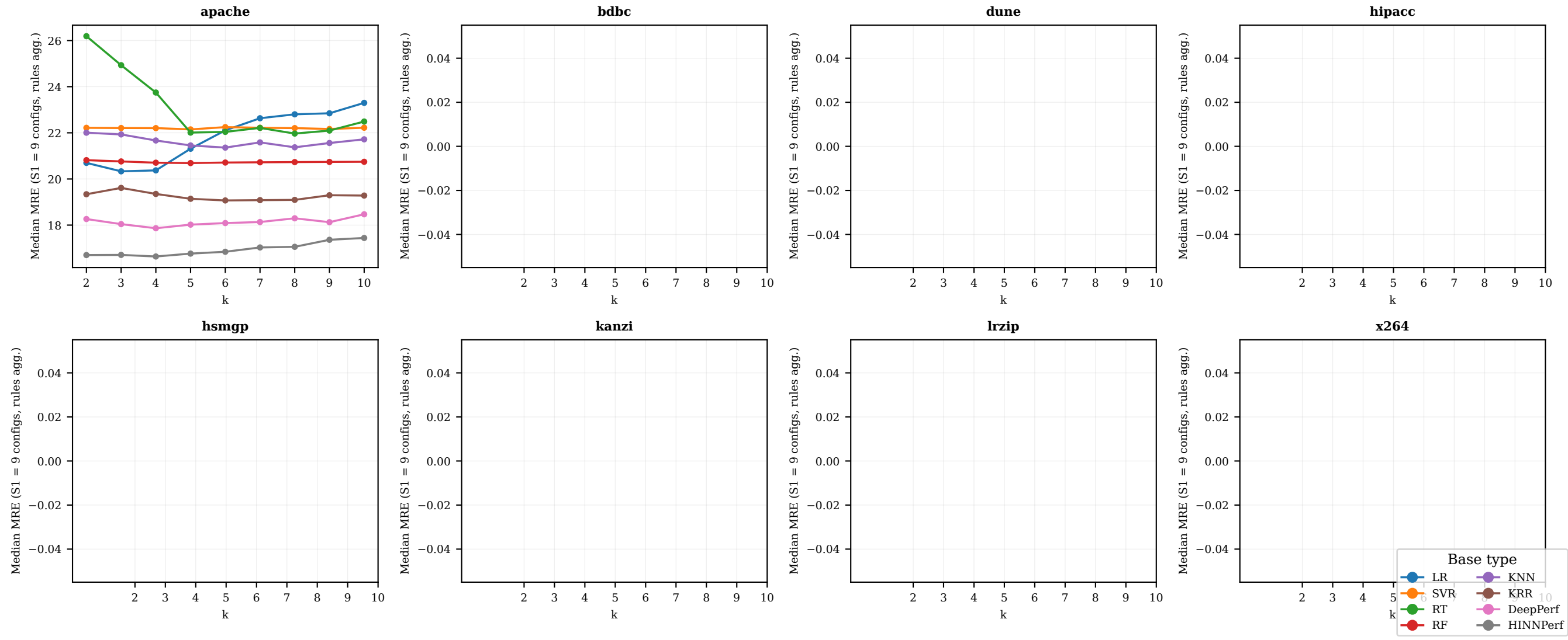
MRE vs k per dataset (S1 only, 9 configs) — 1 line per base type, rules aggregated (RQ3.2)
