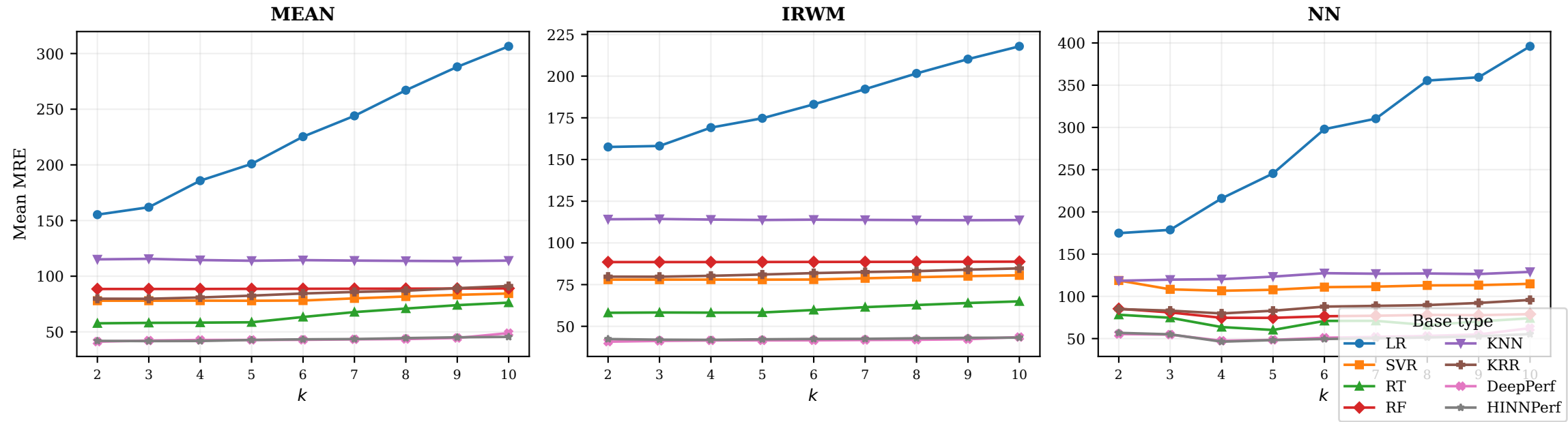
Mean MRE vs. k per rule — 8 base types (S1 per dataset, RQ3.2)
