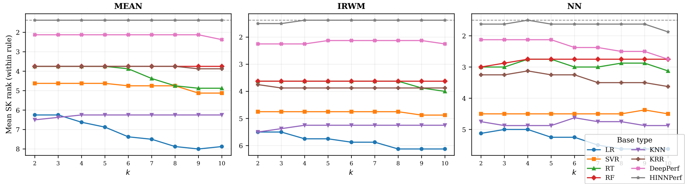
Mean SK rank vs k per rule — 8 base types [perrule] (S1 per dataset, RQ3.2)
