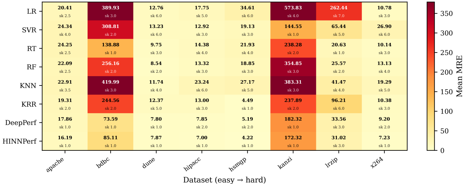
Mean MRE per model \times dataset — S1 only (8 scenarios)
