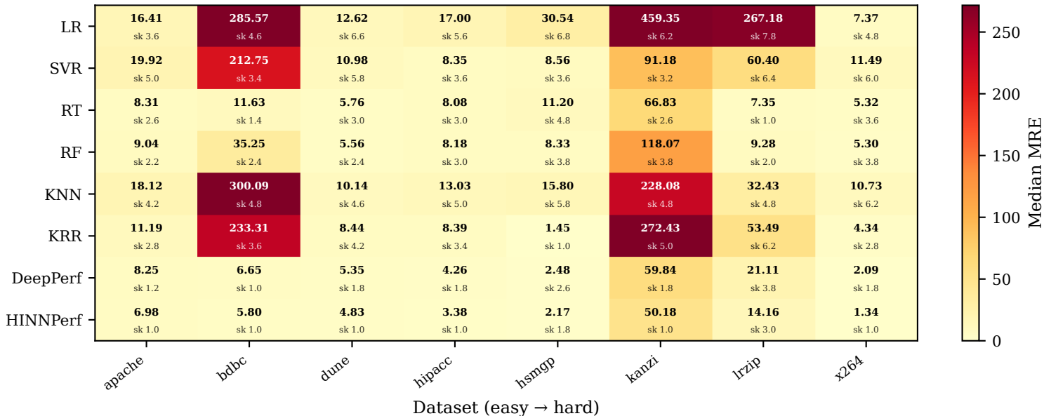
Median MRE per model × dataset — all 40 scenarios
