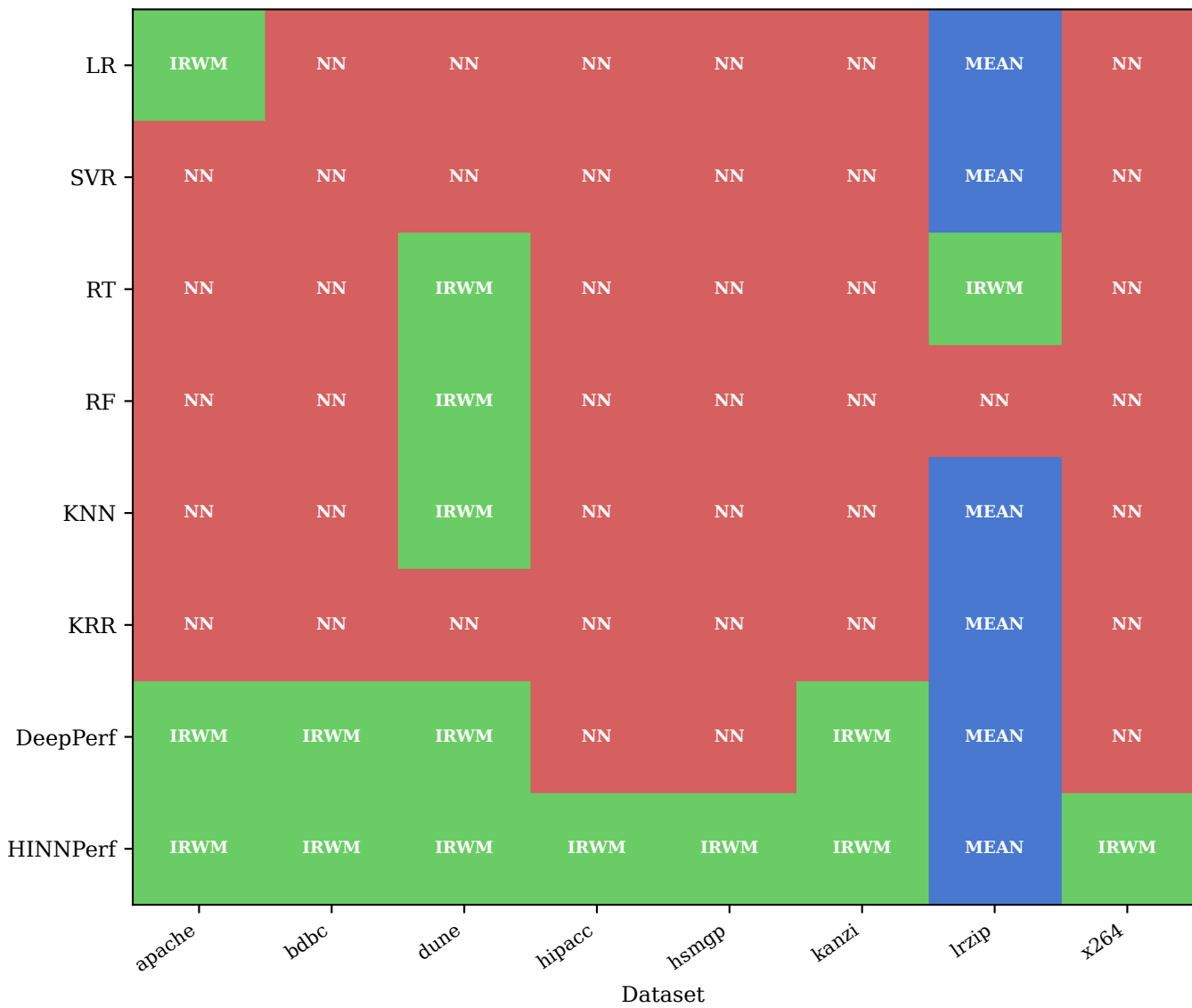
Winning rule per (base type, dataset) — SK rank, S1 (RQ3.3)
