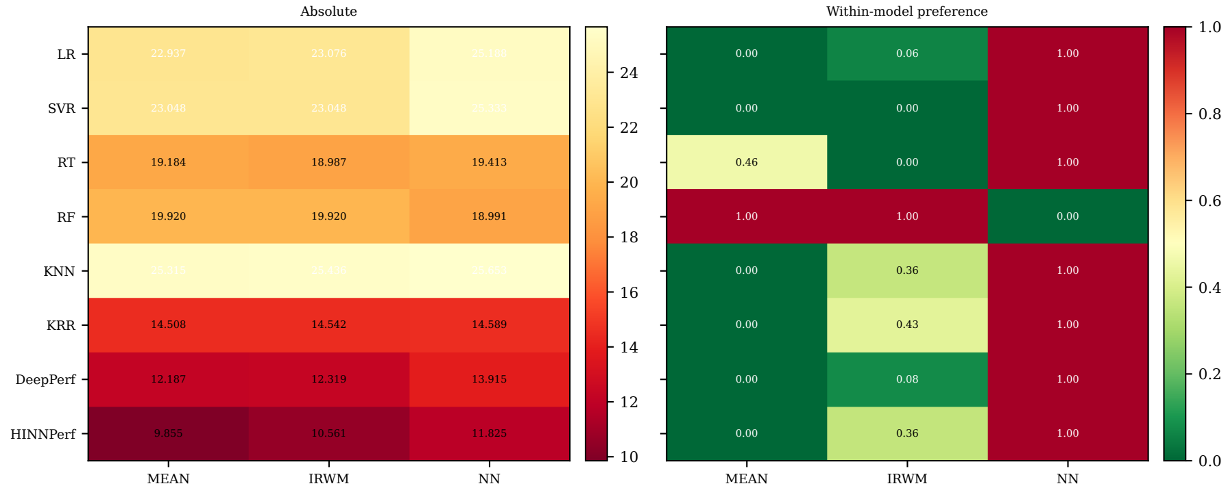
Base-type \times rule interaction — S1 only, median MRE (RQ3.1 / RQ3.3)
