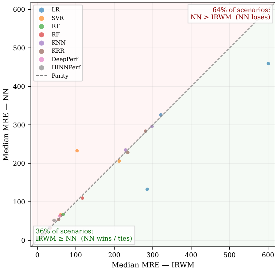
NN vs. IRWM: per-scenario MRE (above diagonal = {rule_b} has higher error \rightarrow {rule_b} loses)
