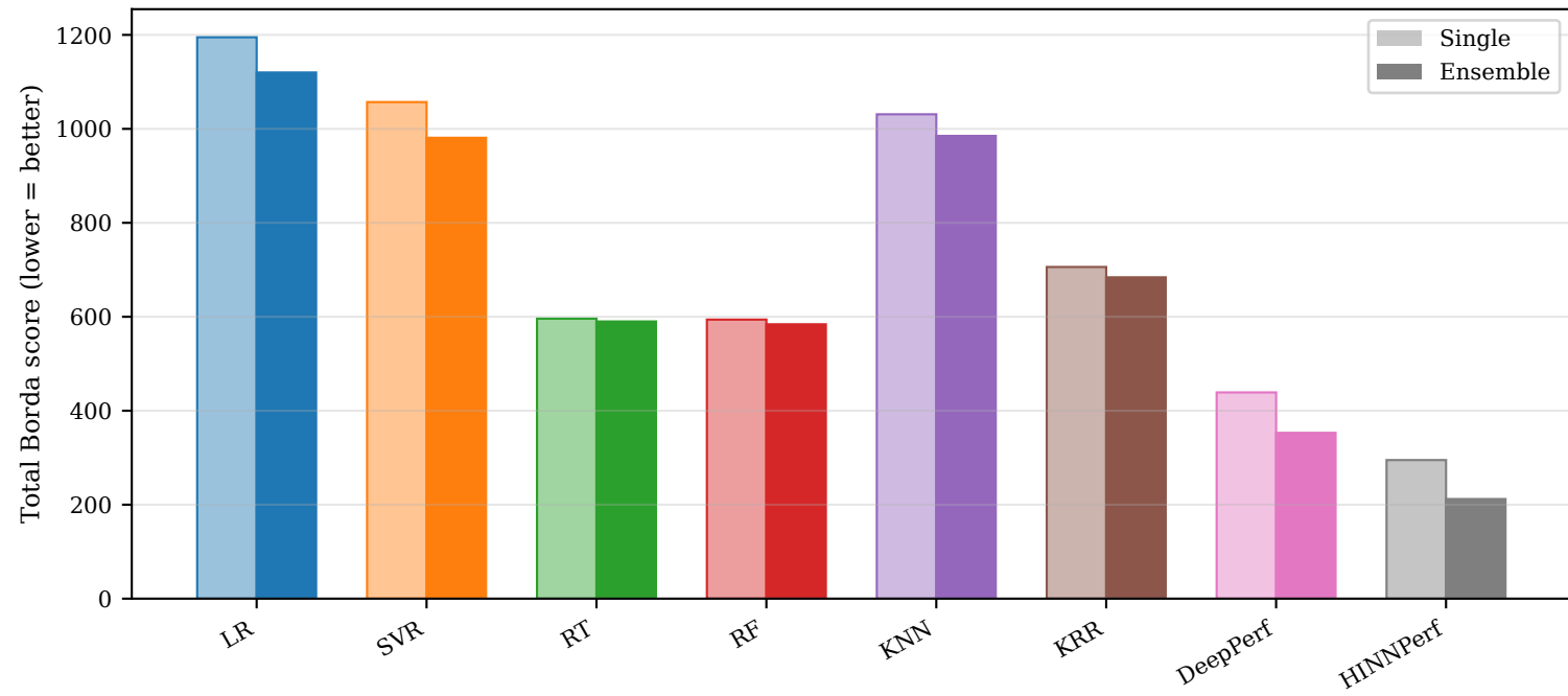
Borda score — singles vs. best ensembles (all 16 competitors together)
