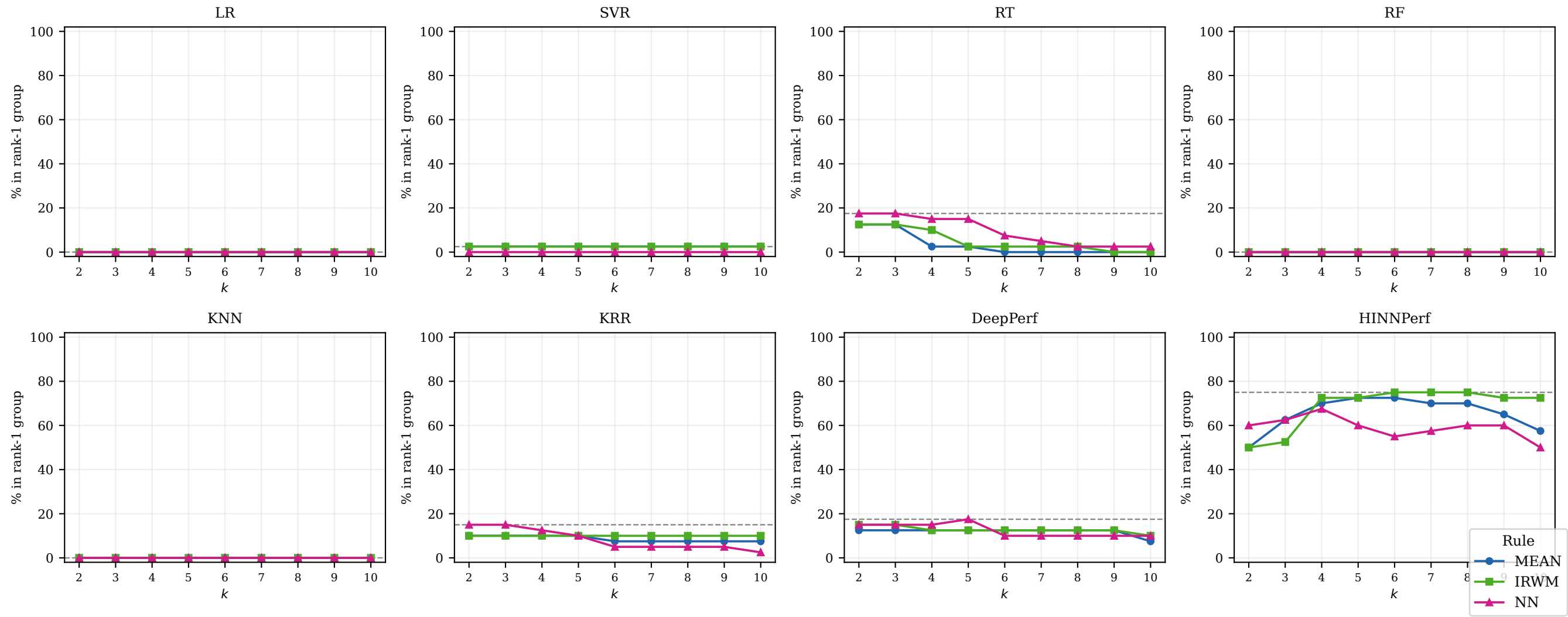
% in best SK group vs k — 40 scenarios [perrule] (RQ3.2) Dashed = best % achieved by this base type across all rules/ k
