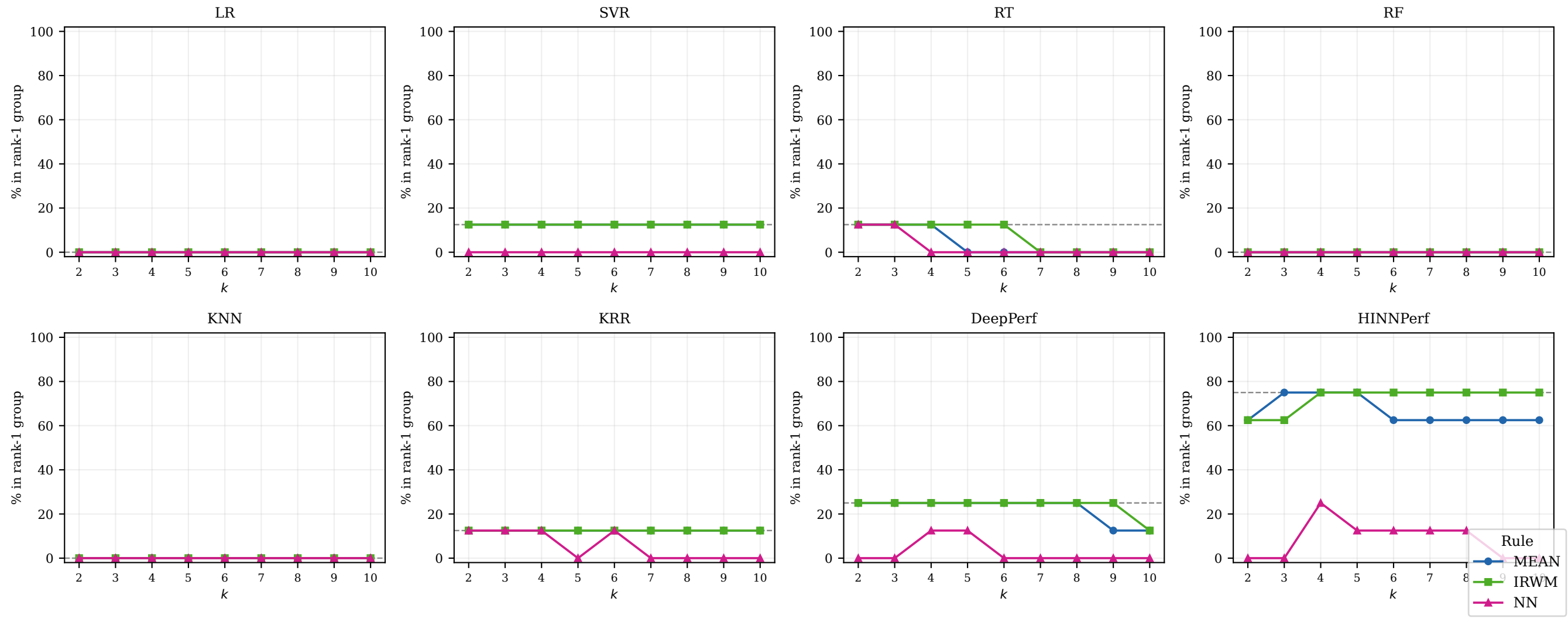
% in best SK group vs k — S1 [global] (RQ3.2) Dashed = best % achieved by this base type across all rules/ k
