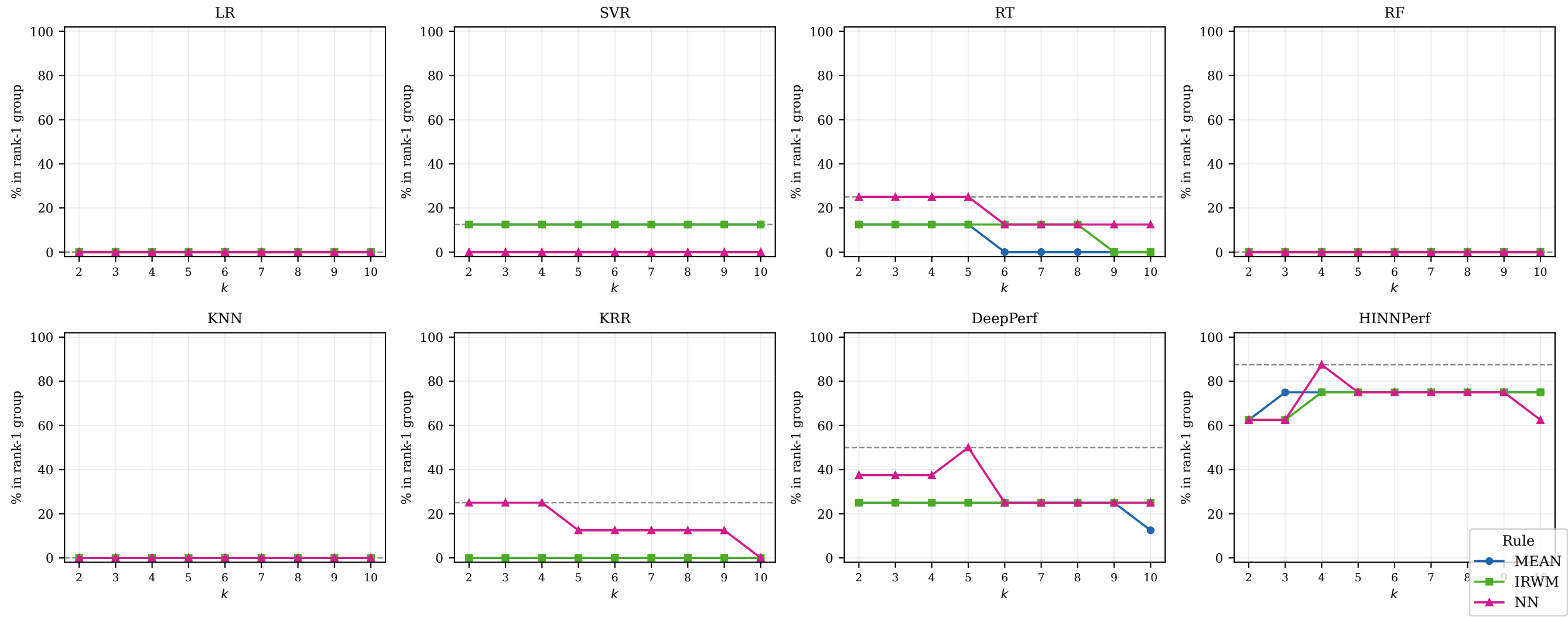
% in best SK group vs k — S1 [perrule] (RQ3.2) Dashed = best % achieved by this base type across all rules/ k
