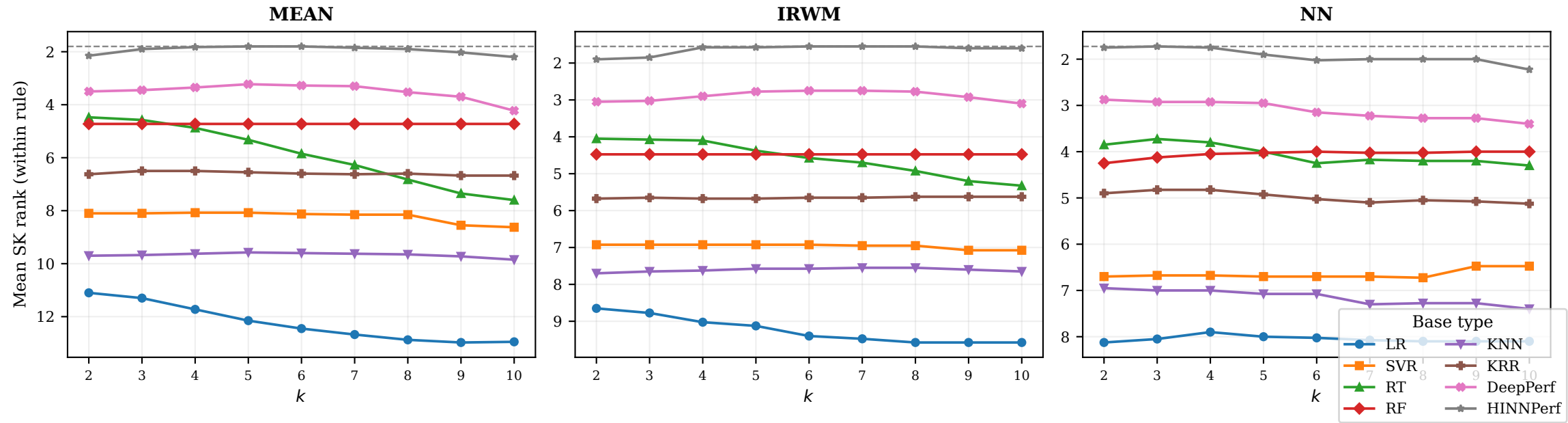
Mean SK rank vs k per rule — 8 base types [perrule] (all 40 scenarios, RQ3.2)
