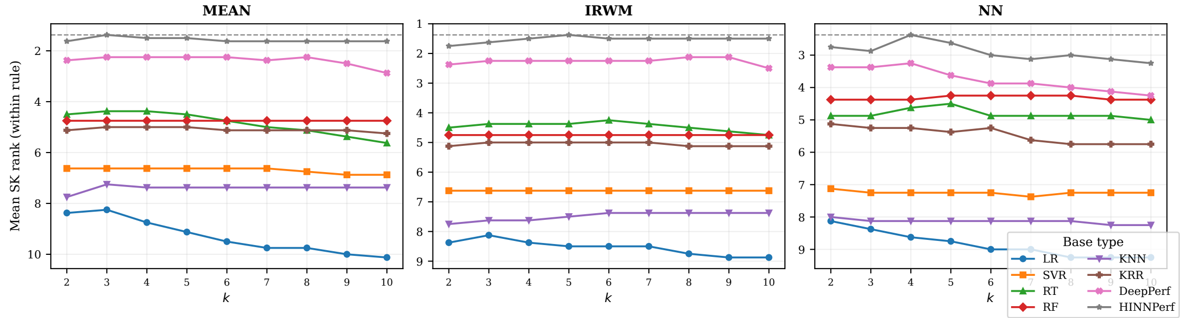
Mean SK rank vs k per rule — 8 base types [global] (S1 per dataset, RQ3.2)
