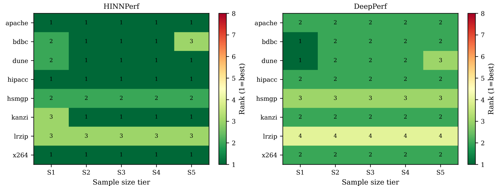
Dataset \times sample-size rank: HINNPerf vs DeepPerf — RQ1
