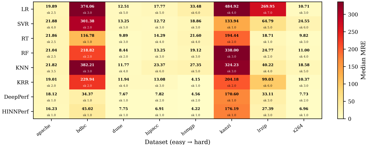
Median MRE per model × dataset — S1 only (8 scenarios)
