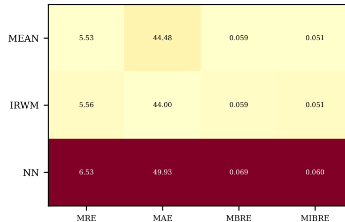
DeepPerf
