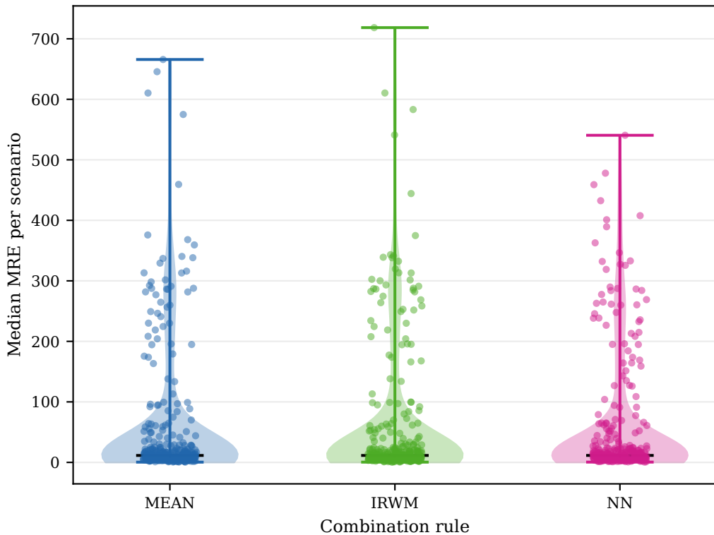
MRE distribution per combination rule (across all base type \times dataset \times sample size scenarios)
