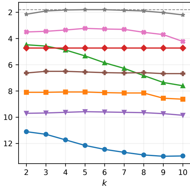
MEAN
