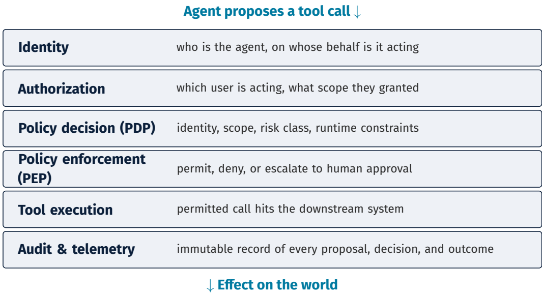
Figure 7.1. The Zero Trust stack for agents. Every tool call descends through identity, authorization, policy decision, enforcement, execution, and audit. No layer is optional.
