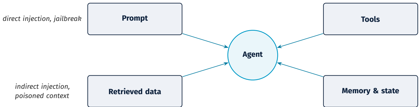
Figure 5.1. The four loci of an agent attack surface — prompt, tools, retrieved data, memory and state — with representative attacks named at each locus.
