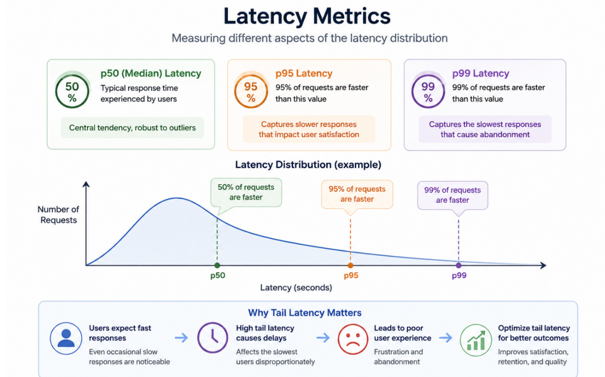
Figure 11.1. Latency metrics: p50/p95/p99 distribution and why tail latency matters for user experience.
