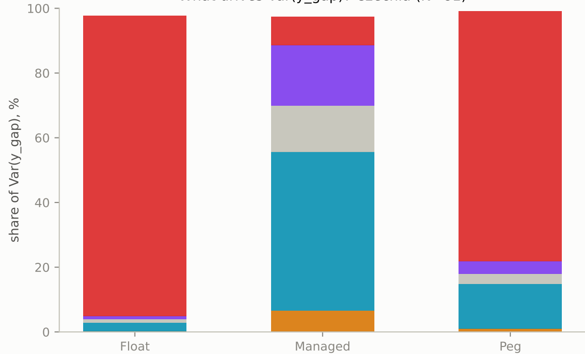
What drives \text{Var}(y_{\text{gap}}) ? Czechia (N=81)
