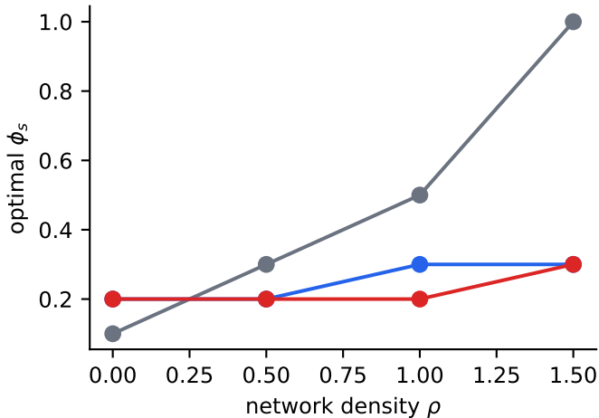
Optimal FX weight ( \phi_\pi = 20 , \phi_y = 1 )
