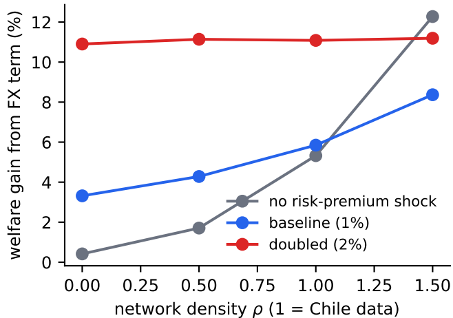
Value of responding to the exchange rate
