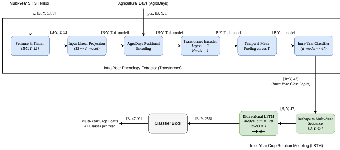
Figure 2.4: Hierarchical overview of the Transformer-LSTM architecture, demonstrating the fusion of intra-year attention and inter-year recurrence.
