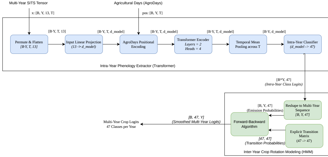
Figure 2.3: Hierarchical overview of the Transformer-HMM cascade, demonstrating the fusion of intra-year attention and inter-year transition modeling.
