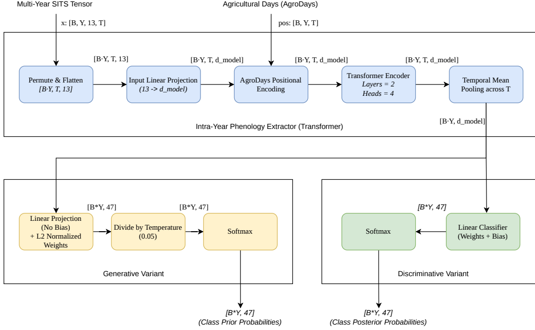
Figure 2.2: Architectural block diagram of the standalone Transformer Encoder (Generative and Discriminative variants).
