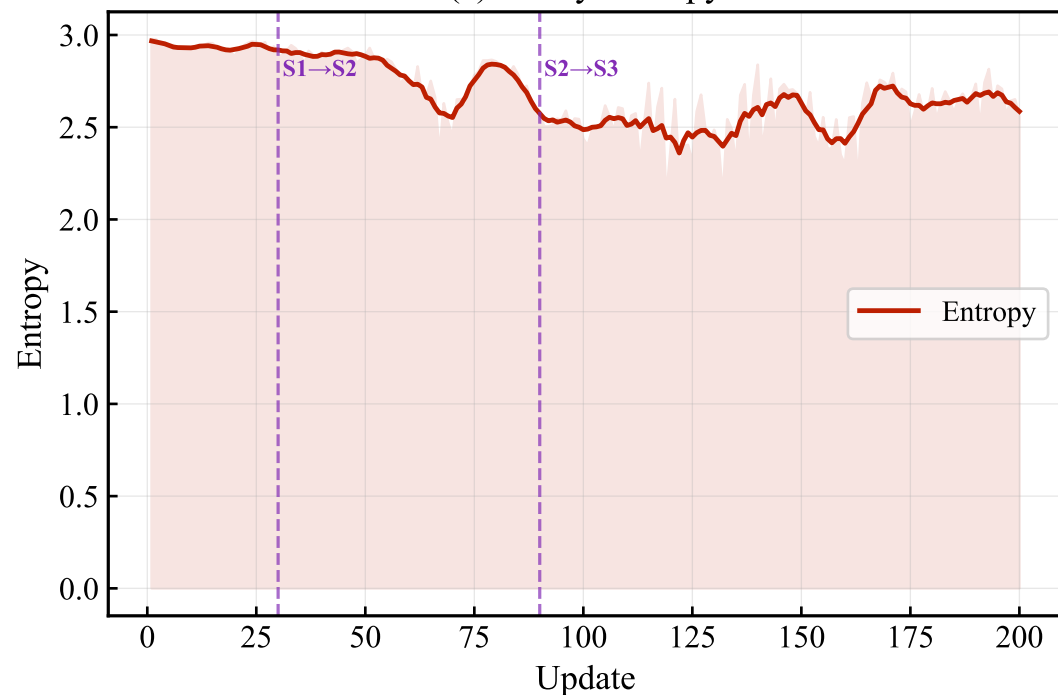
(c) Policy Entropy
