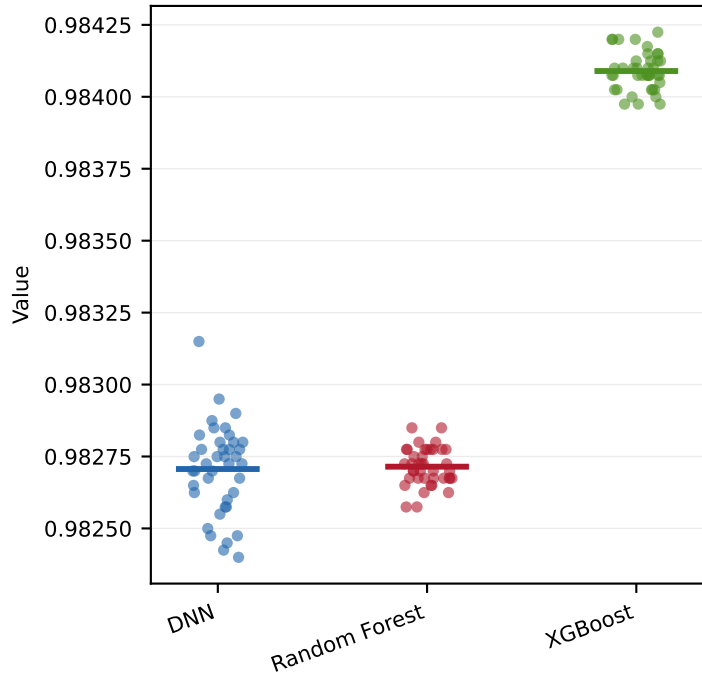
Aggregate accuracy
