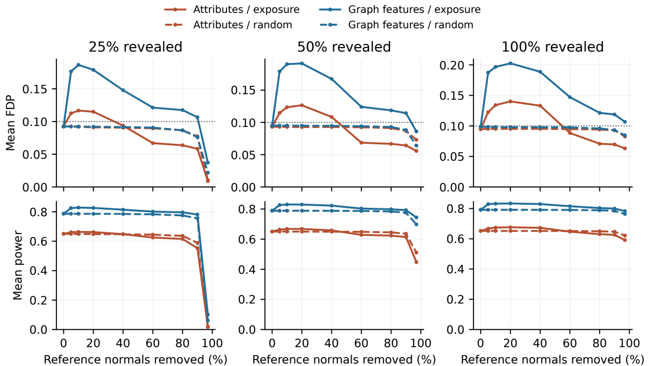
Figure 7: T-Finance: complete prespecified removal sweep. Both scorers, all nine removal fractions and all three revelation fractions are shown. Solid lines use exposure removal; dashed lines use equally sized random references. Means retain every abstention and average ten training-seed means.
