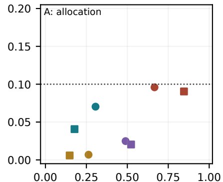
Weibo (GADBench)
