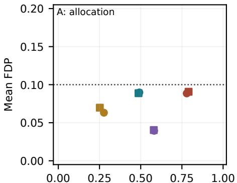
Amazon
