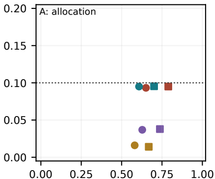
T-Finance
