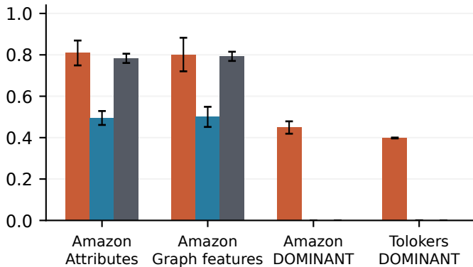
Mean power
