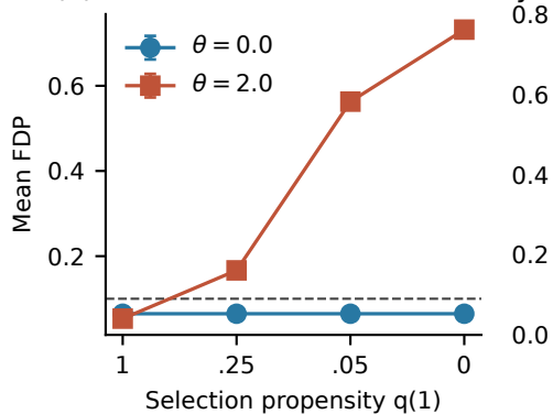
(a) Selection and score sensitivity
