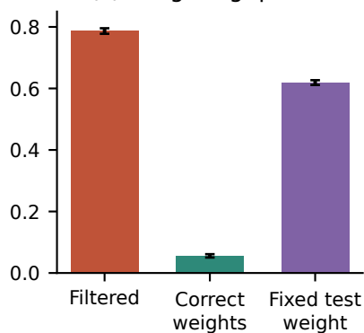
(c) Weighting: power
