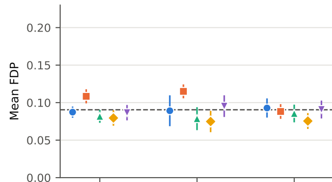
Amazon
