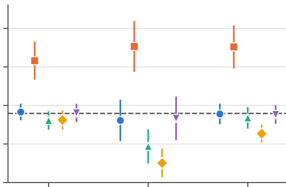
Weibo (GADBench)
