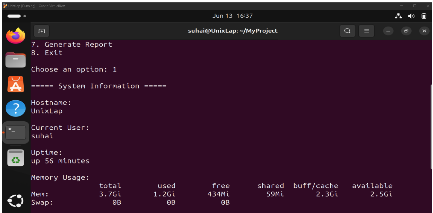
Figure 2: System Information 2
