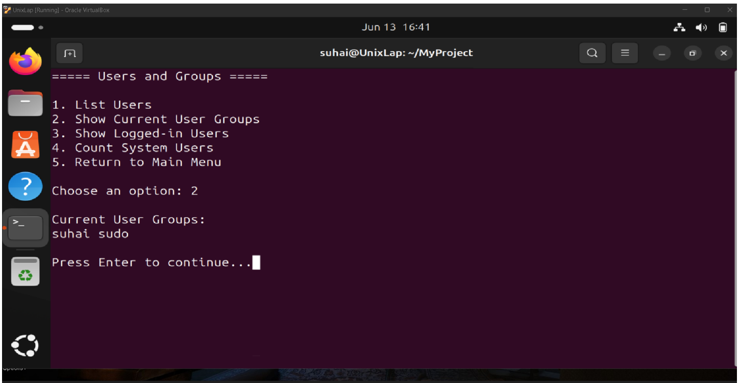
Figure 7: Users & Groups 4
