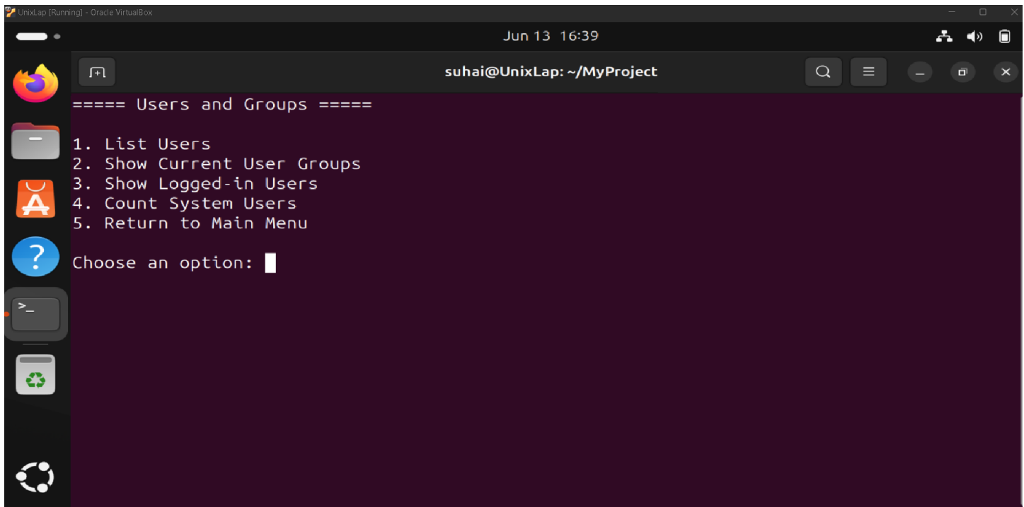
Figure 4: Users & Groups 1
