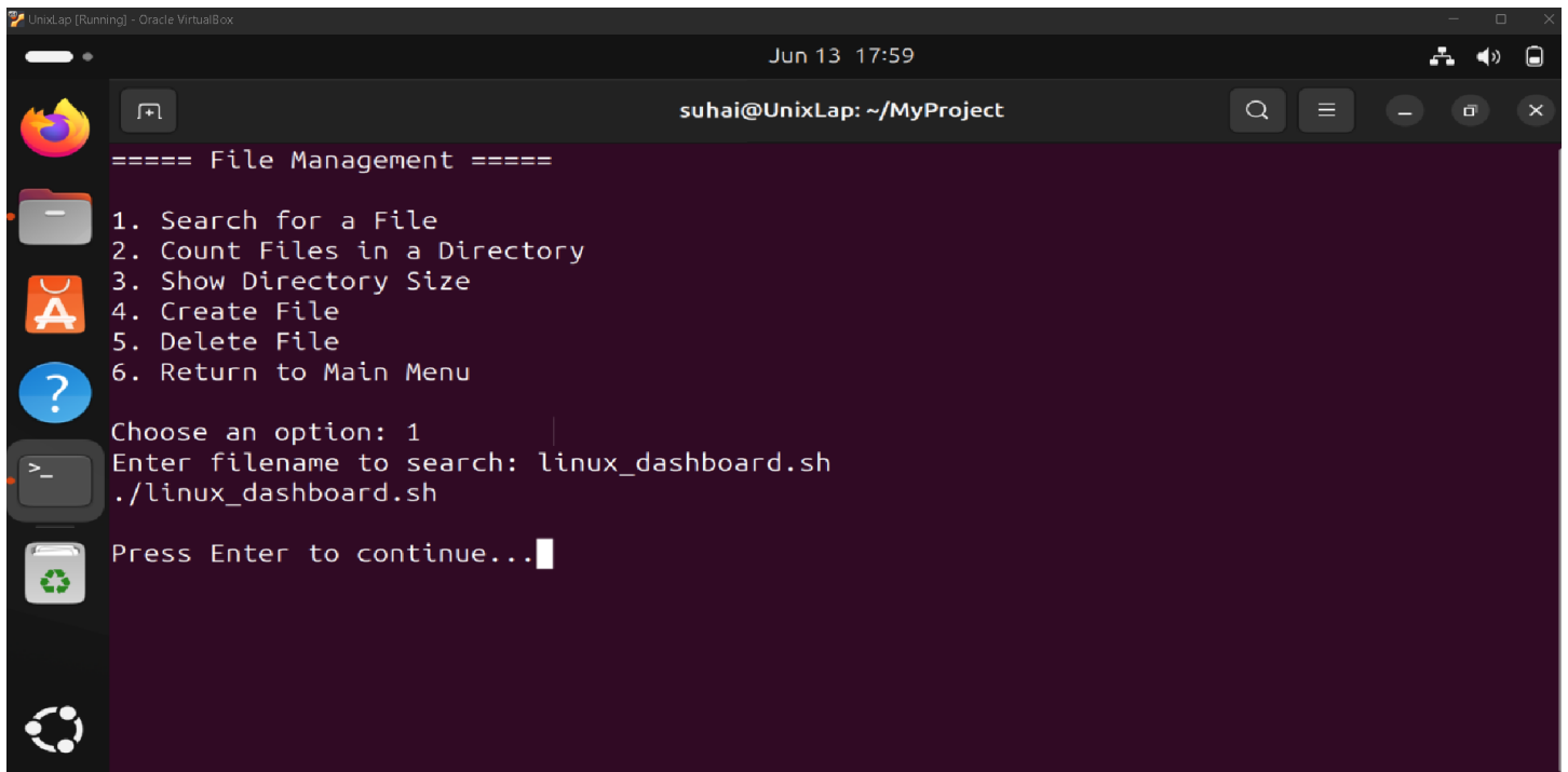
Figure 10: File Management 1
