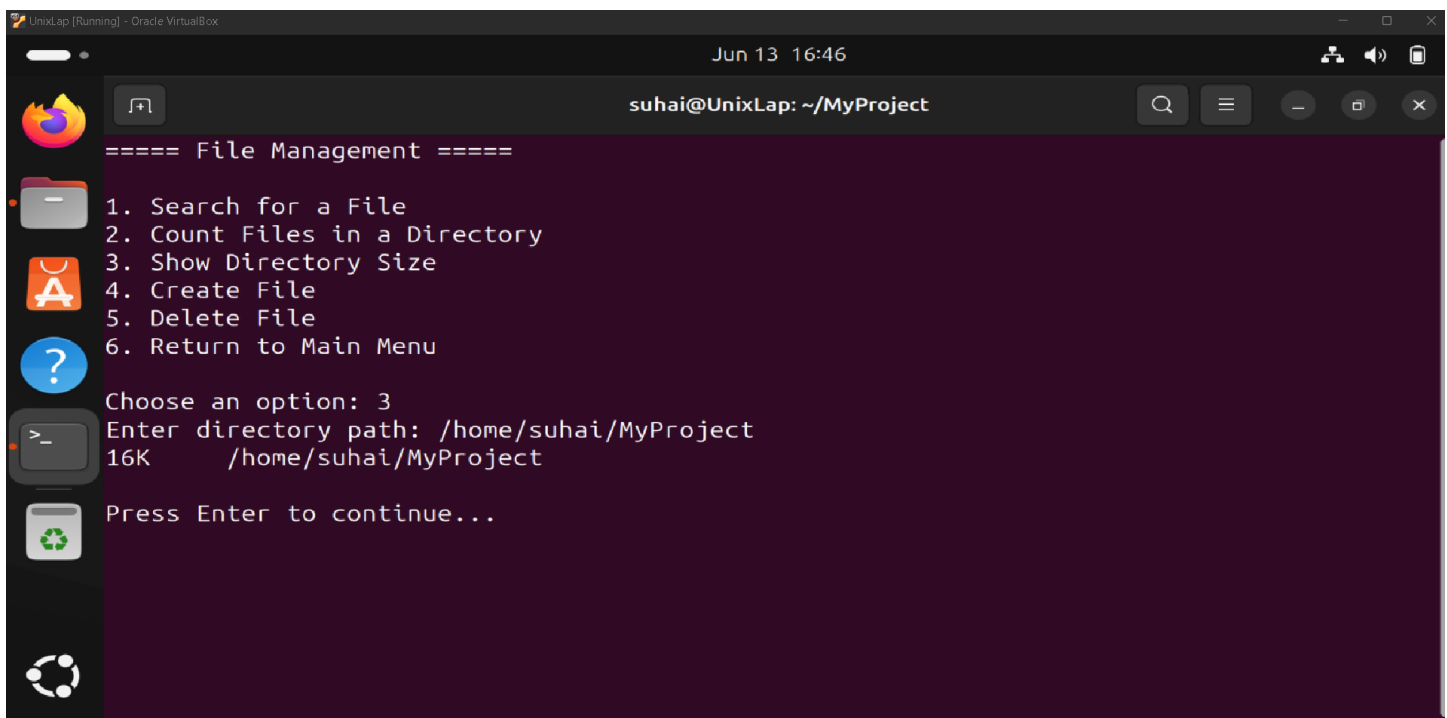
Figure 12: File Management 3
