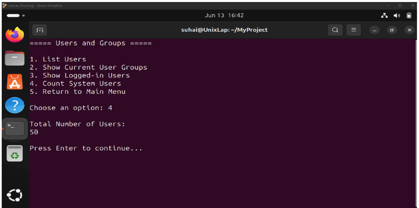
Figure 9: Users & Groups 6
