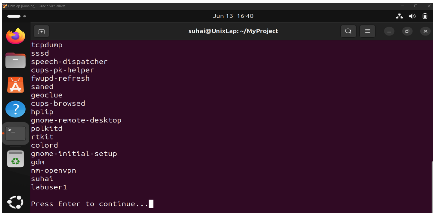
Figure 6: Users & Groups 3
