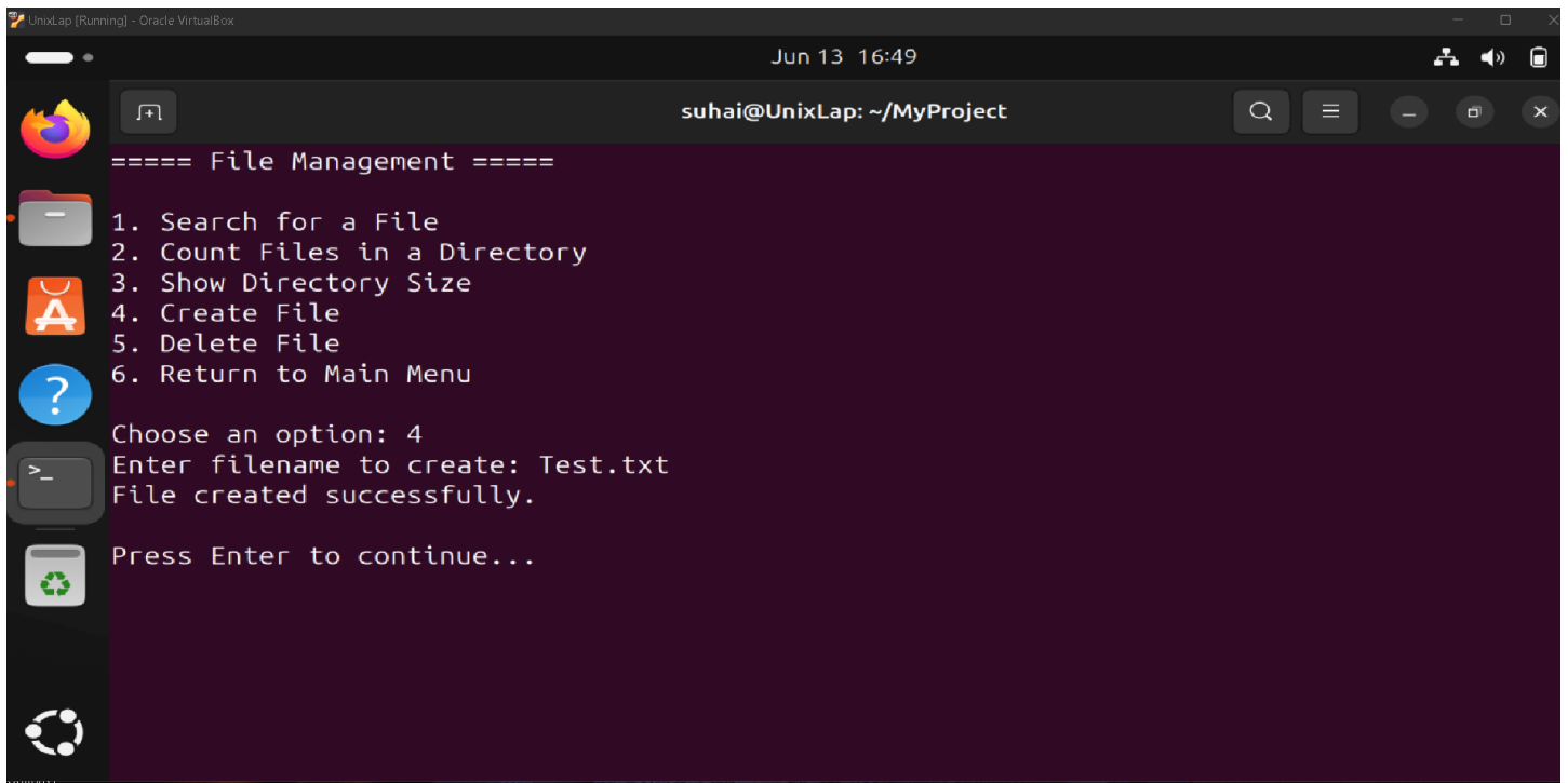
Figure 13: File Management 4
