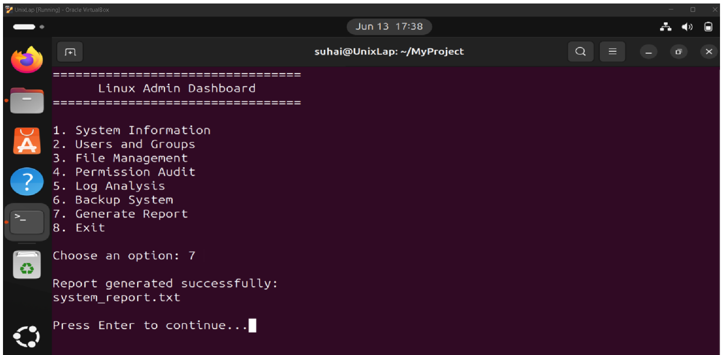
Figure 20: Generate Report
