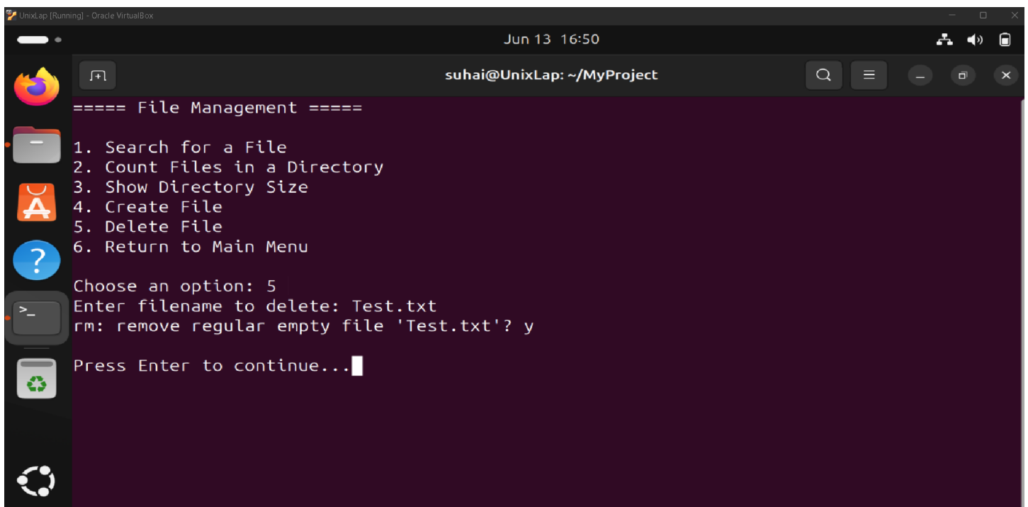
Figure 14: File Management 5
