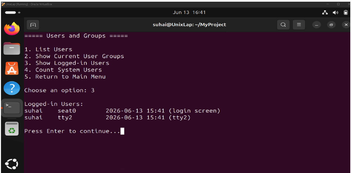
Figure 8: Users & Groups 5
