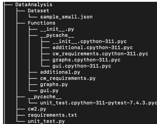
Figure 12: Directory structure in a tree format.
