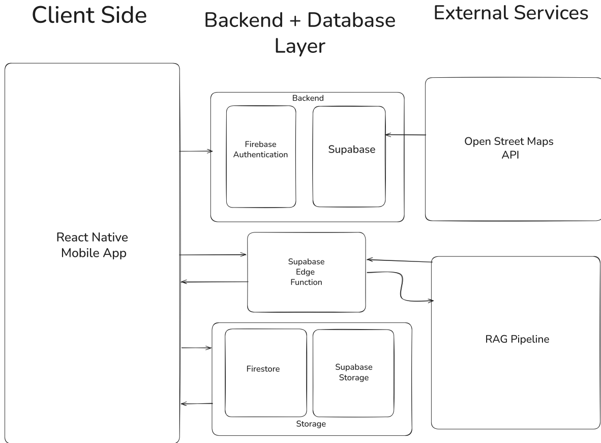
Figure 4.1: System Architecture of EdumentX
