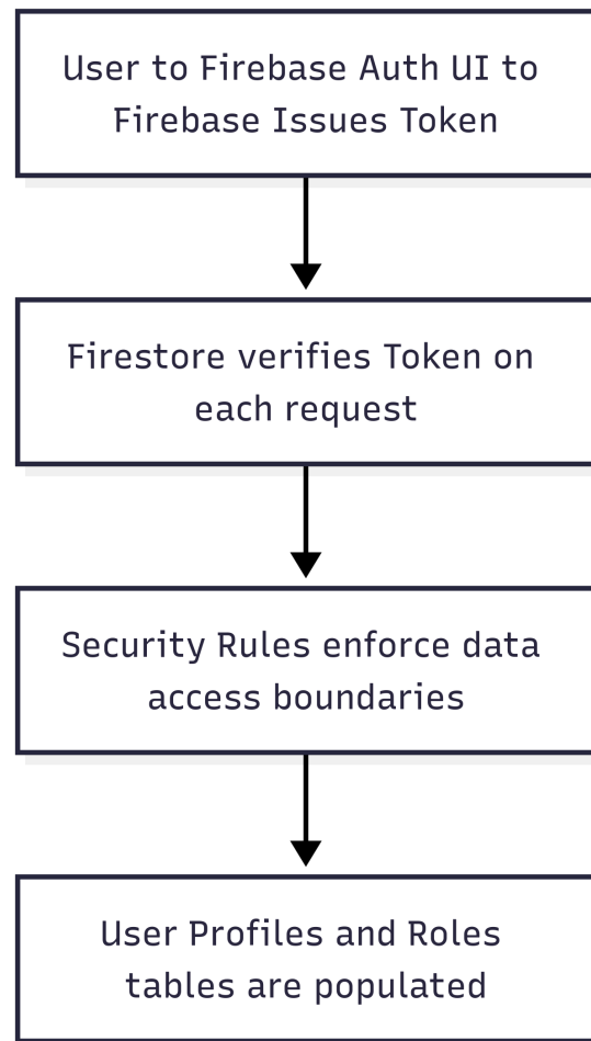
Figure 3.1: Authentication and Onboarding Workflow
