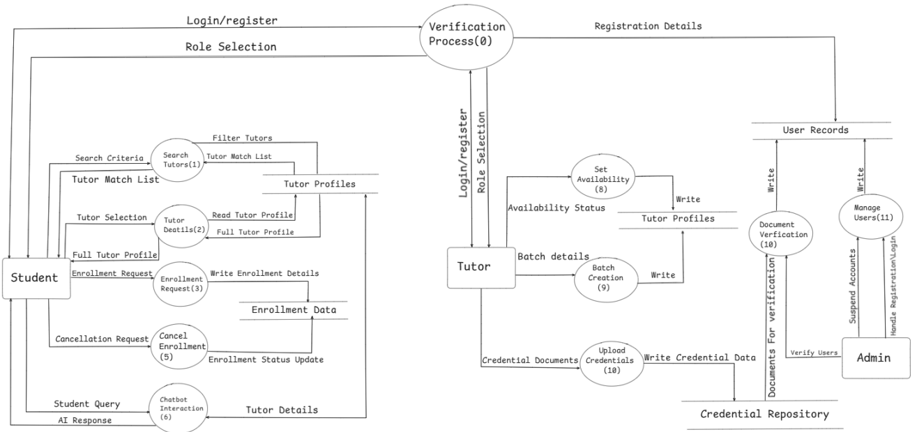
Figure 4.3: Level 1 Data Flow Diagram
