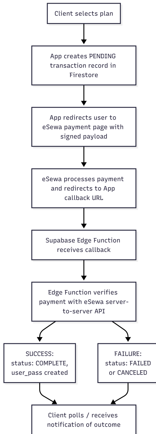
Figure 3.4: eSewa Payment Transaction Flow
