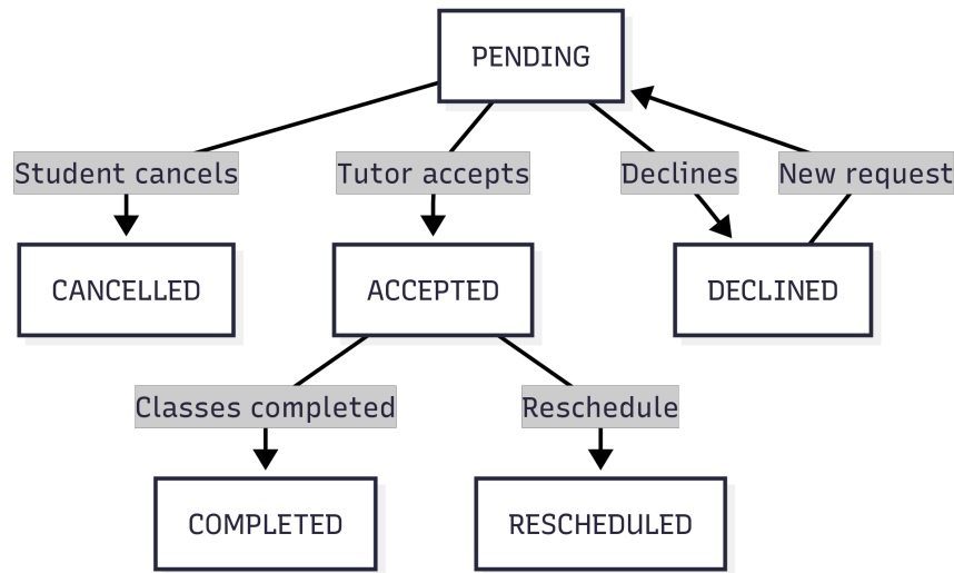
Figure 3.3: Enrollment Request Status Lifecycle
