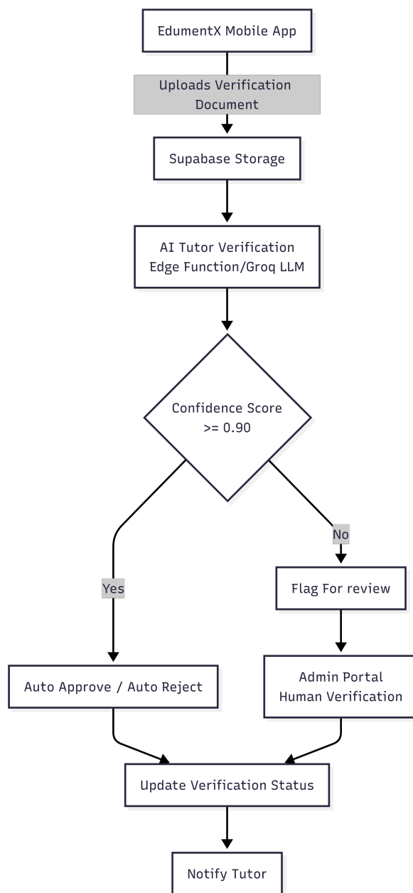
Figure 3.2: Architecture of Tutor Verification Process
