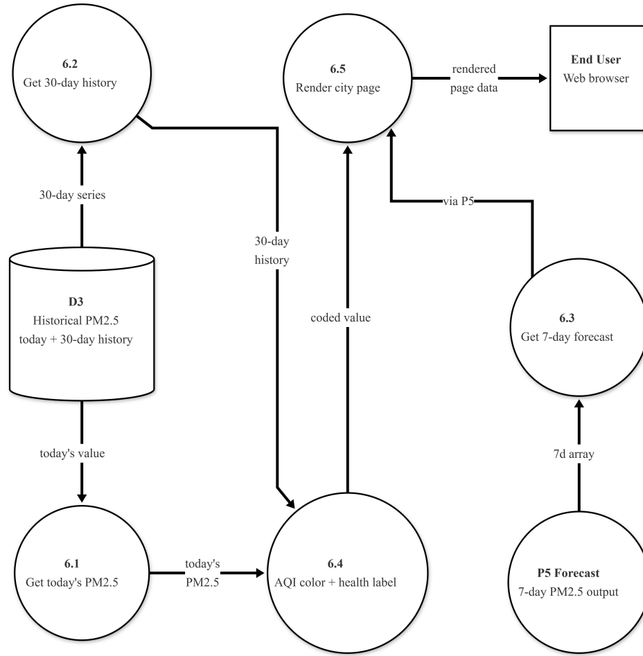
Figure 4.10: DFD - Level 2.6: Frontend Update
