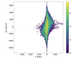
Figure 3. This is the observed velocity plotted as a function of radius and the circular velocity of the merger remnant edge on.
